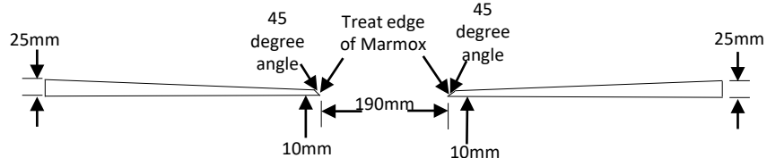
CROSS SECTION A
